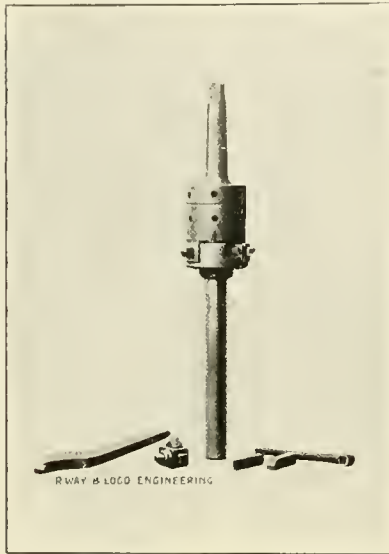
FIG. 3. MICROMETER BORING BAR FOR LATHE.
